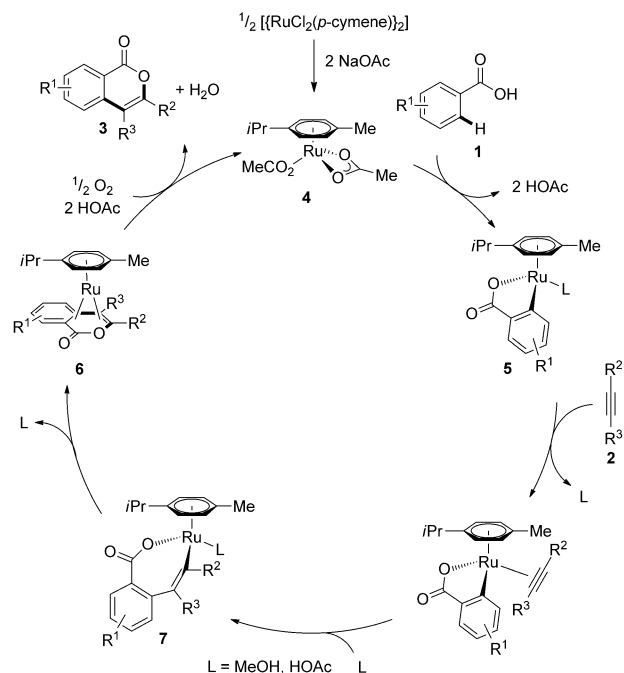
Scheme 6. Proposed catalytic cycle for alkyne annulation with oxygen.
