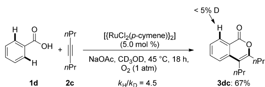
Scheme 3. Studies highlighting the rate-determining C–H ruthenation.
