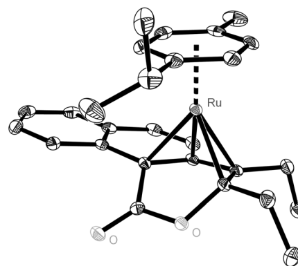
Figure 2. Molecular structure of complex 6f . H atoms are omitted for clarity. Anisotropic displacement parameters are depicted at the 50% probability level.
