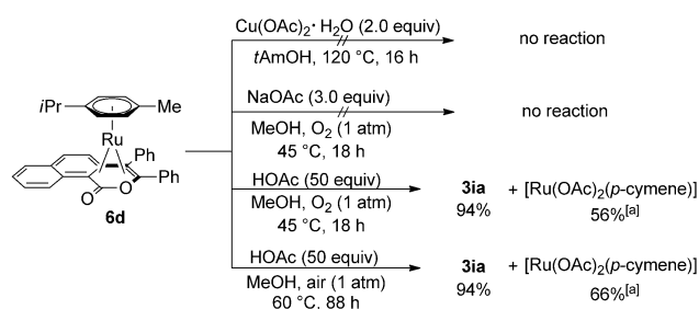
Scheme 5. Oxidation of ruthenium(0) complexes 6 . [a] Determined by ^1\text{H} NMR spectroscopy using 1,4-dimethoxybenzene as an internal standard.
