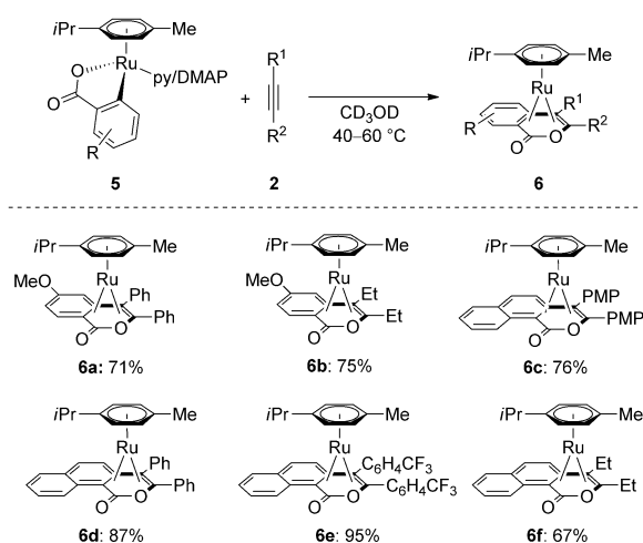
Scheme 4. Transformation of ruthena(II)cycles 5 with alkynes 2 as monitored by ^1\text{H} NMR spectroscopy using 1,4-dimethoxybenzene as an internal standard.
