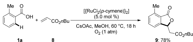
Scheme 7. Aerobic ruthenium(II)-catalyzed annulation of alkene 8 .
