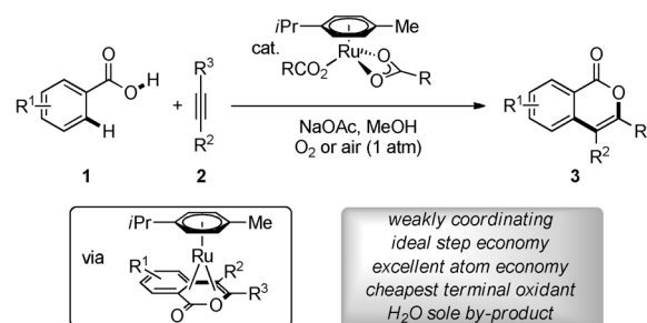
Figure 1. C–H activation of weakly coordinating benzoic acids 1 with O 2 .
