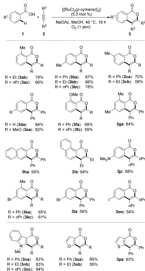
Scheme 1. Scope of the aerobic ruthenium(II)-catalyzed alkyne annulation.
