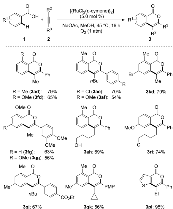
Scheme 2. Aerobic ruthenium(II)-catalyzed C–H activation with unsymmetrical alkynes 2 .
